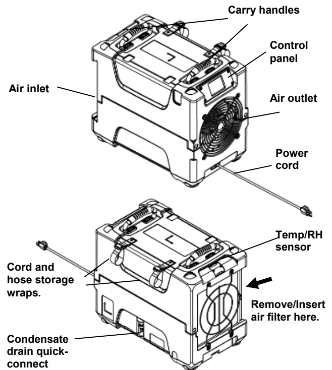
Fig. A: Parts Identification
