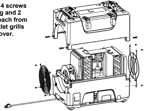
Fig. B: Disassembly for Cleaning
